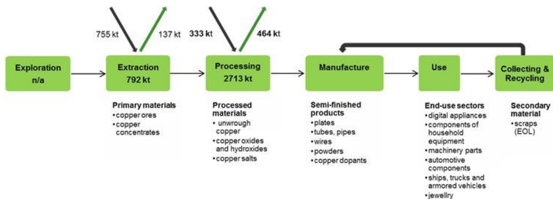
Figure 53: Simplified value chain for copper in the EU, average 2012-2016 44
